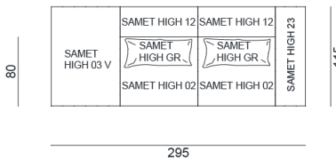
Samet High Configuration N
