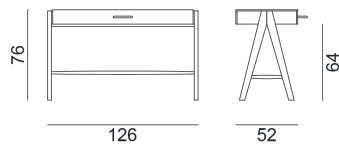
Pier 60
